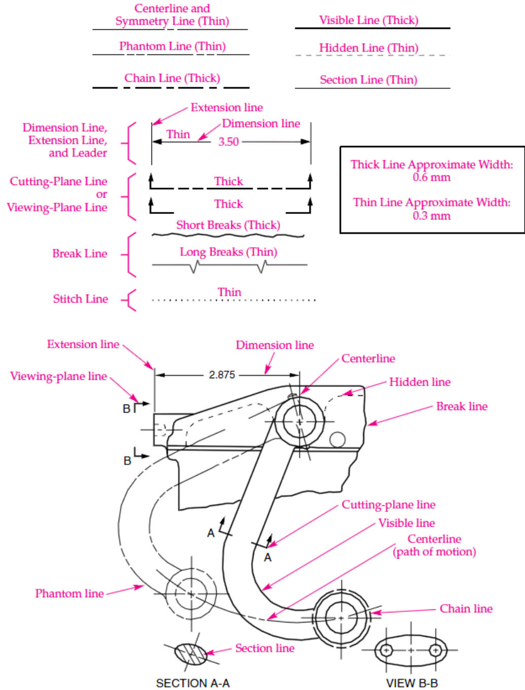
Figure 3-1. Line conventions. (Adapted from ASME Y14.2M)
